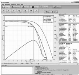
PV-Analysator, Kennlinie
